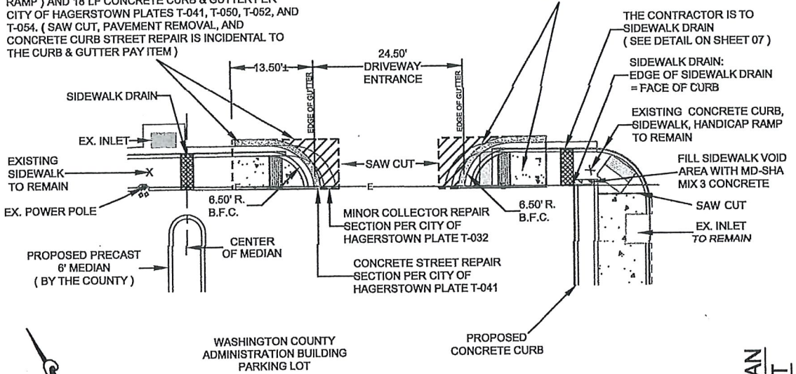
ENTRANCE - 1 SCALE: 1" = 10' ( BY THE CONTRACTOR )
