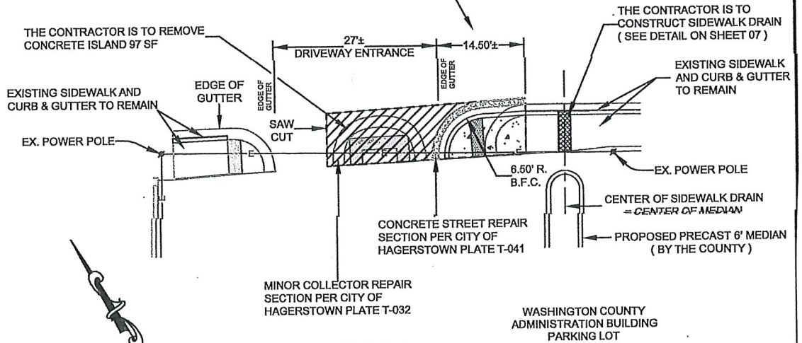
ENTRANCE - 3 SCALE: 1" = 10' ( BY THE CONTRACTOR )
