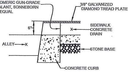
SECTION - "D" NTS
