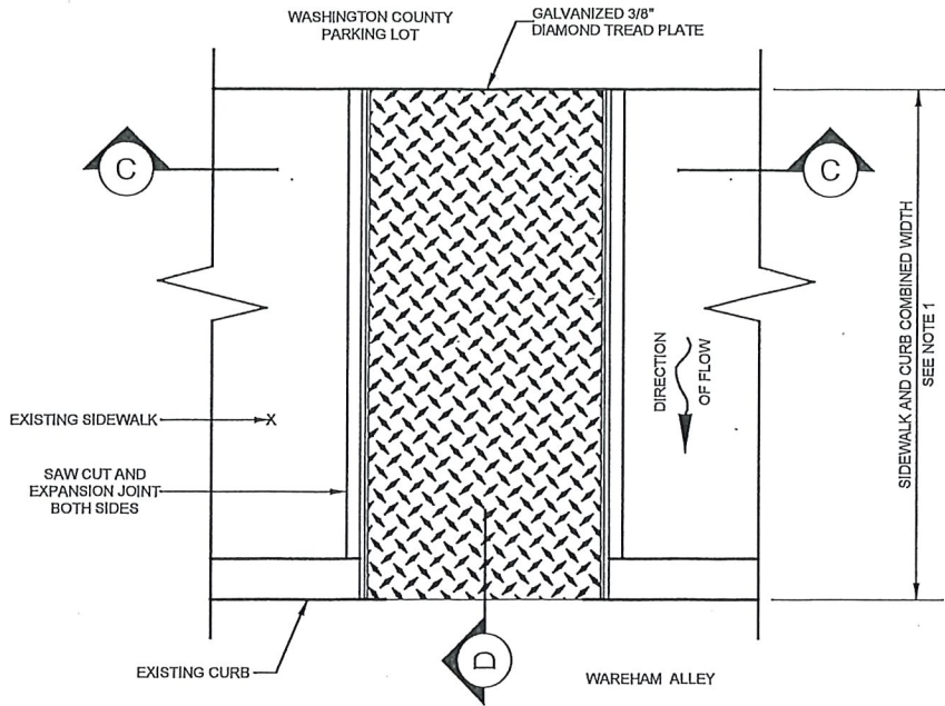
SIDEWALK DRAIN TOP VIEW NTS
